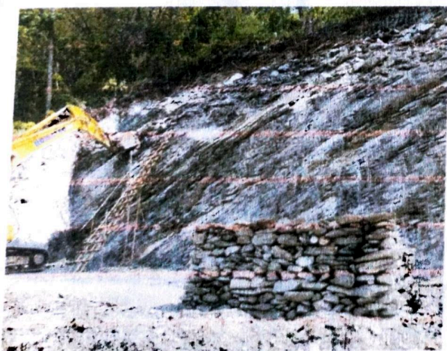
Rock slope netting
