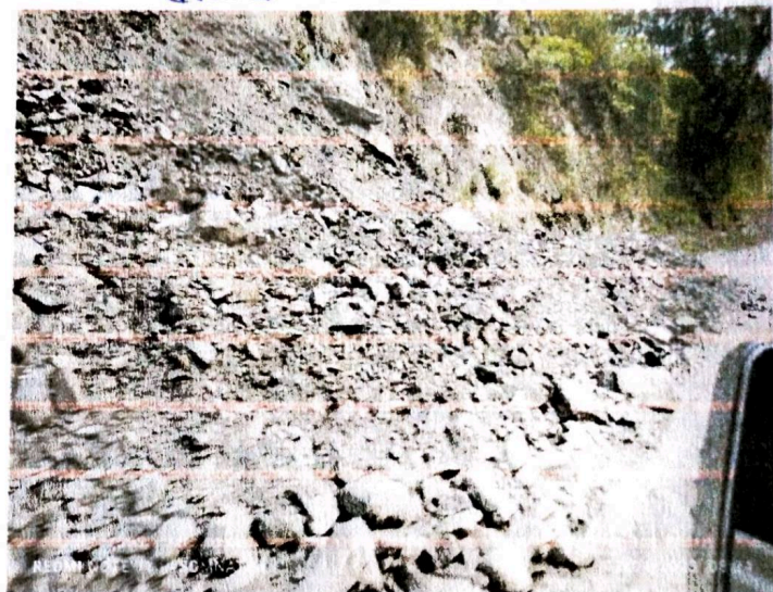
Land subsidence
